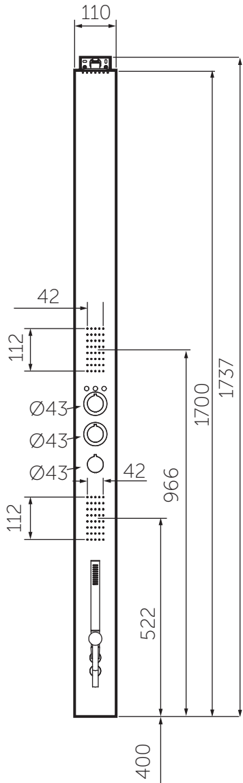
VISTA FRONTAL
